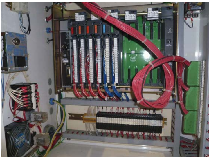
CABINET WIRING
