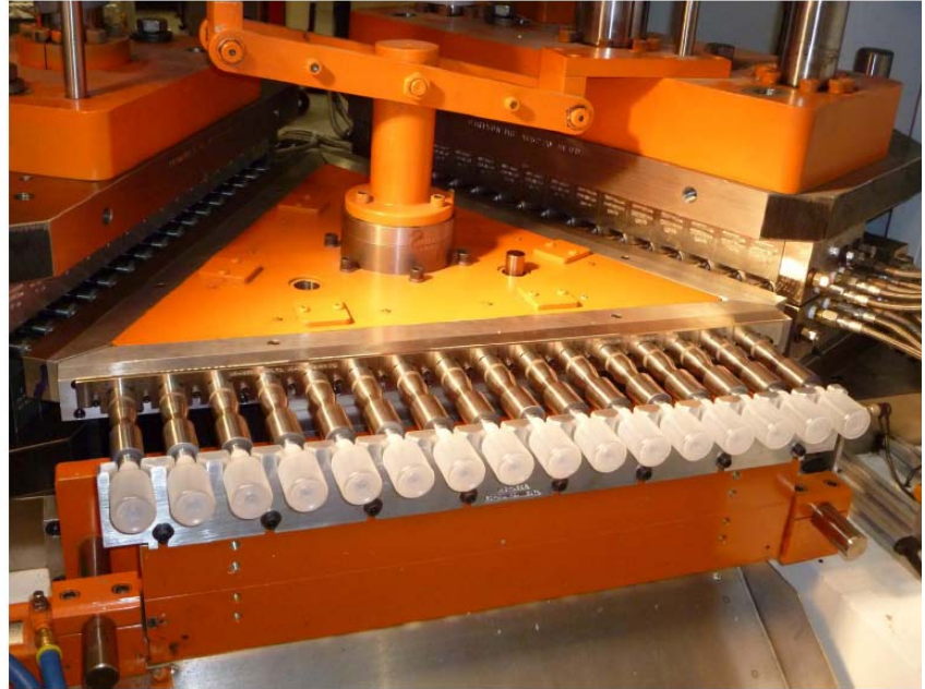
Jomar Model 85S LDPE Dropper Bottle, 16 cavities
